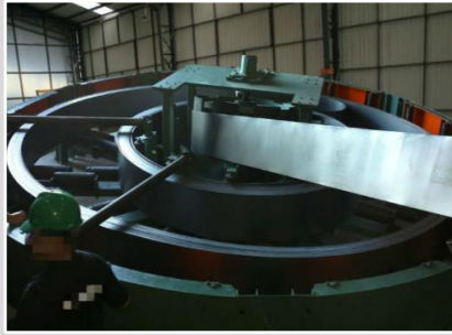
Horizontal Roller Accumulator for tube sizes of \phi 76 - \phi 114\text{mm}
