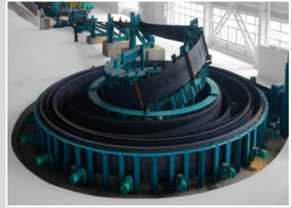
Horizontal Spiral Accumulator for tube sizes of > \phi 165\text{mm}
